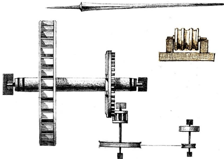
Fig. 256 Sword blade, grinding train and grinding stone
